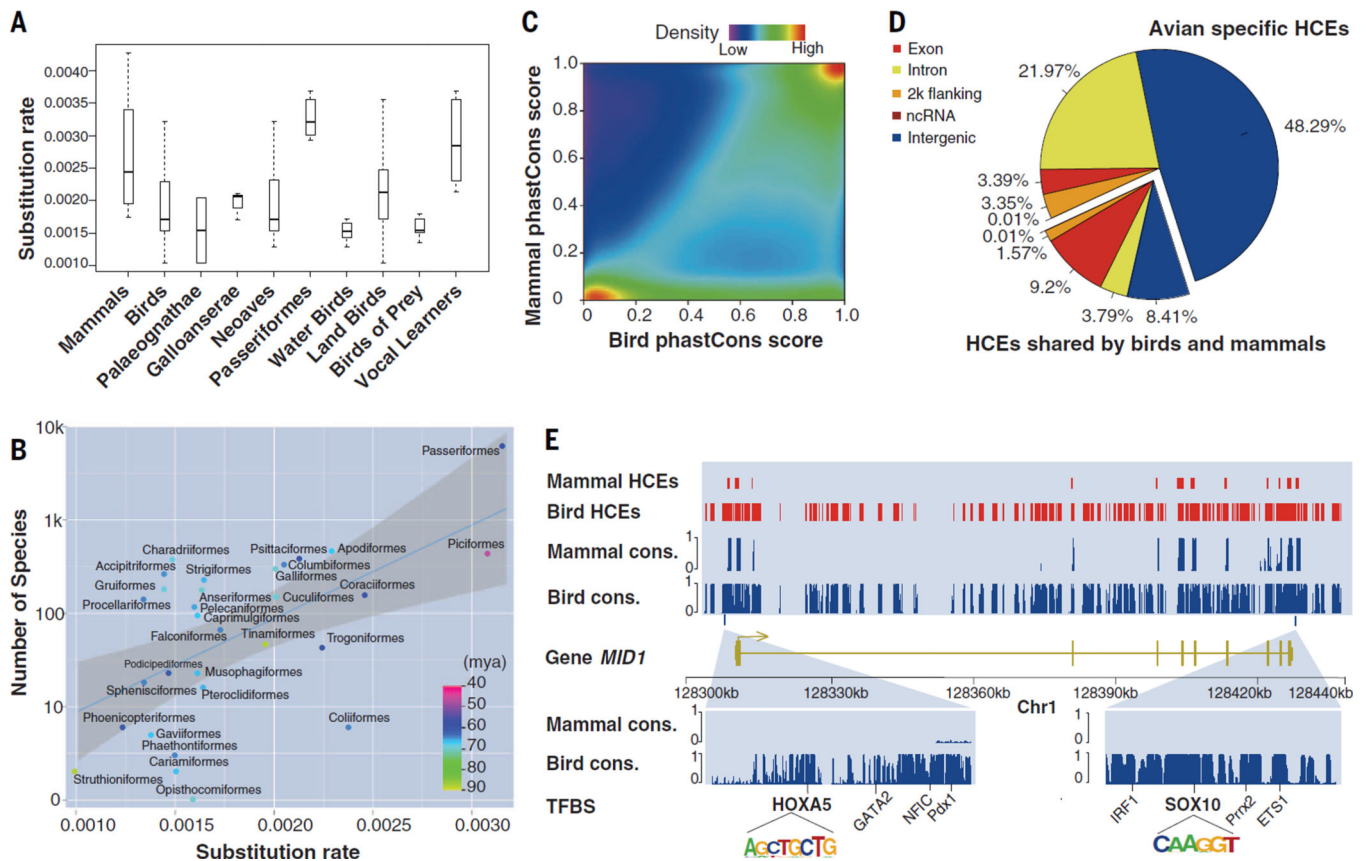
Fig. 3. Evolutionary rate and selection constraints
