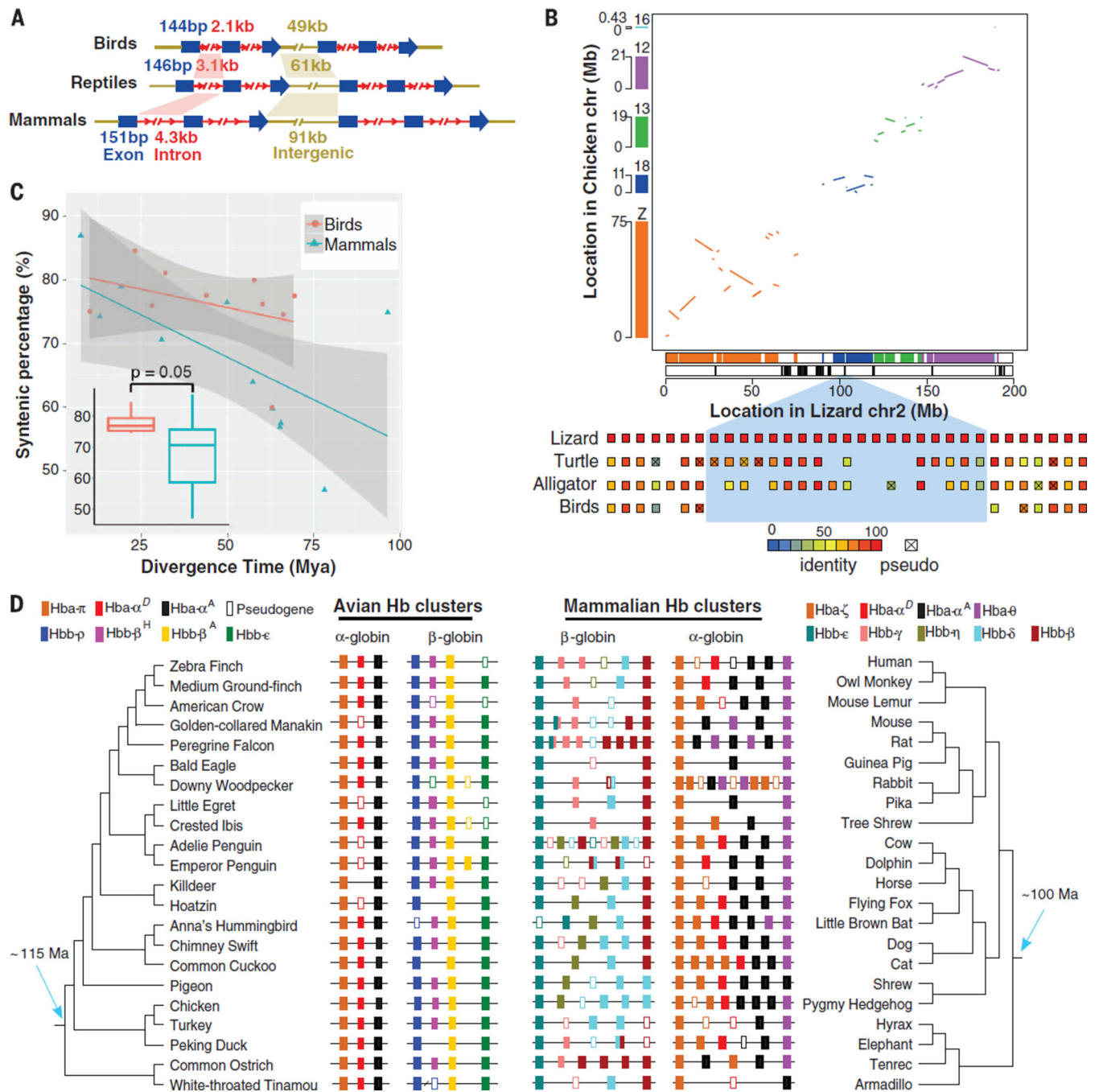
Fig. 2. Genome reduction and conservation in birds
