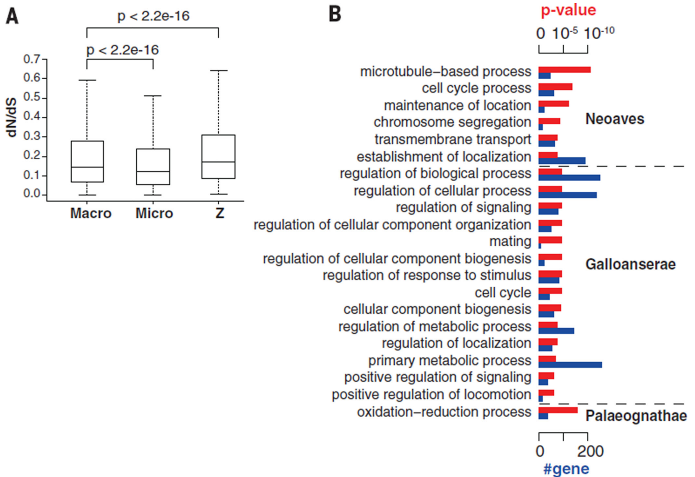
Fig. 4. Selection constraints on genes
