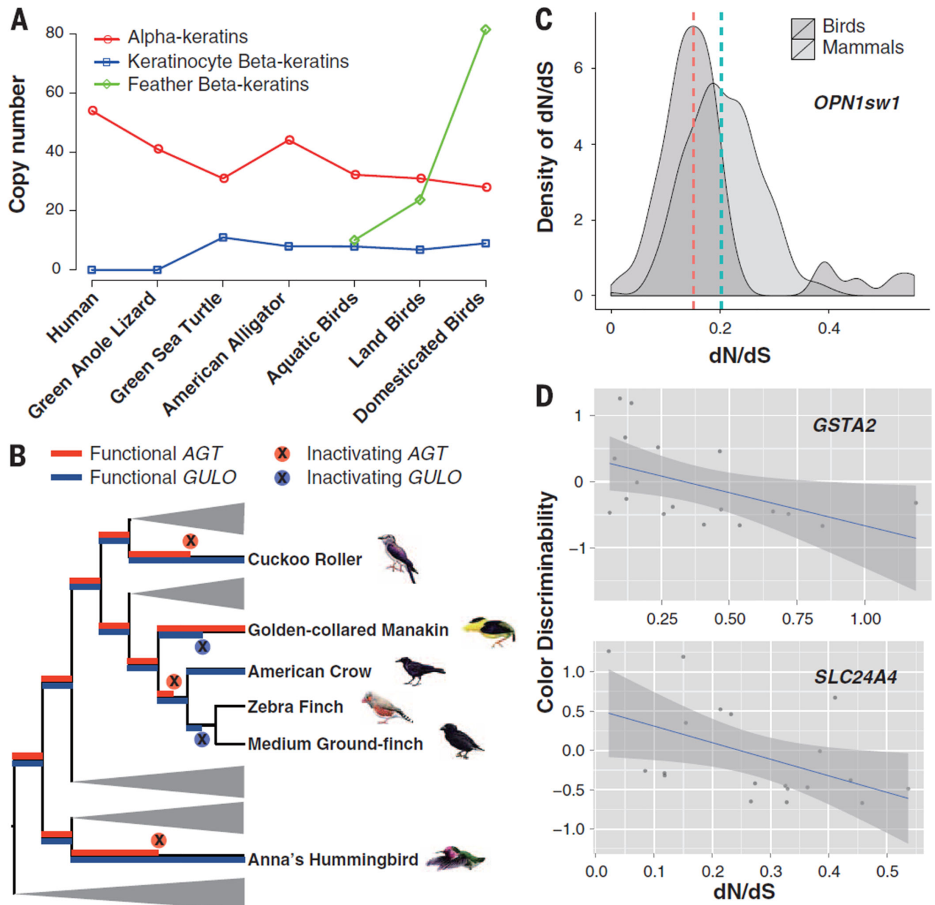
Fig. 6. Genetic changes associated with ecological adaptations
