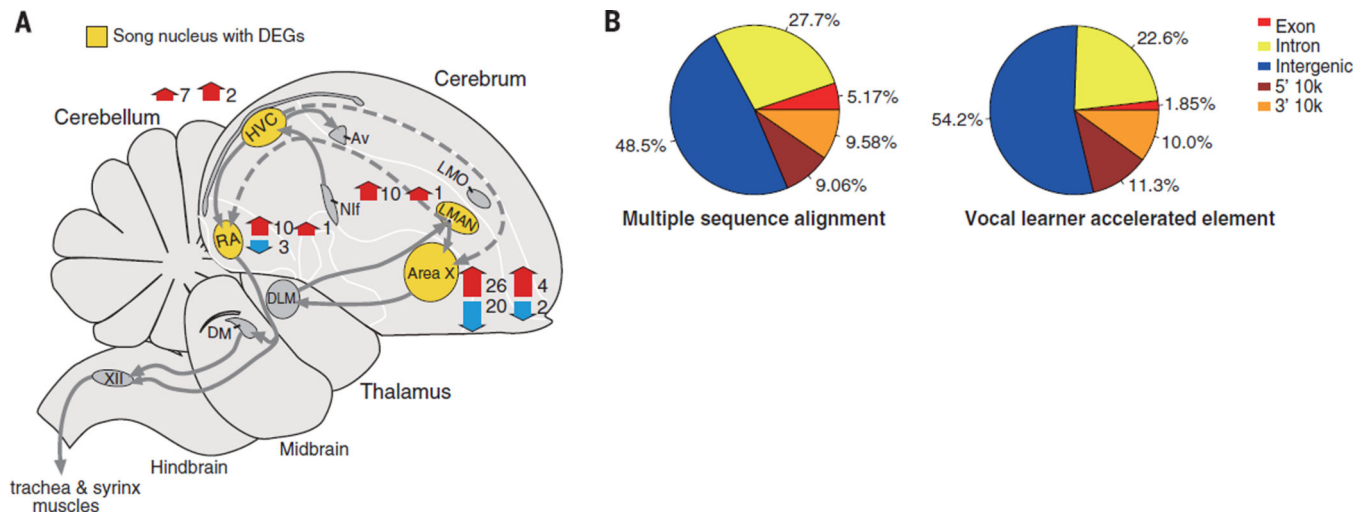
Fig. 5. Convergent molecular changes among vocal learning birds
