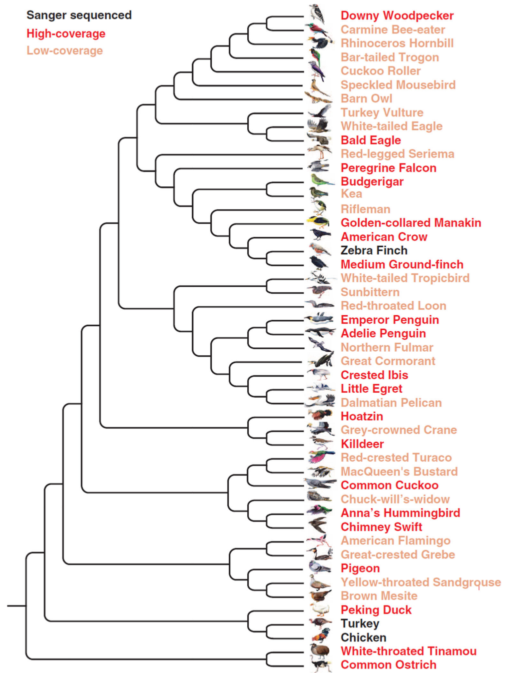
Fig. 1. Avian family tree and genomes sequenced
