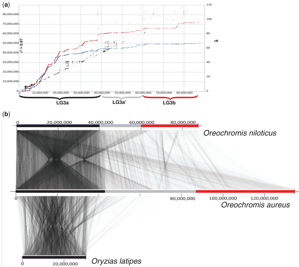
Fig. 3. Patterns of recombination in Oreochromis niloticus correspond to the organization of synteny between O. niloticus and O. aureus LG3. (a) Recombination of female (red) and male (blue) O. niloticus LG3 shown in cM (right) and linkage disequilibrium ( r^2 > 0.97 , left) in black. Adapted with permission from (Conte et al. 2019). (b) Syntenic relationships of the 87-Mb anchored assembly of LG3 in O. niloticus , compared with the 134-Mb anchored assembly of LG3 in O. aureus , compared with the ancestral chromosome 18 in Oryzias latipes .
